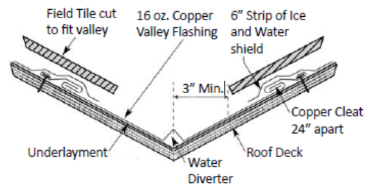
↑ Example of an open valley
