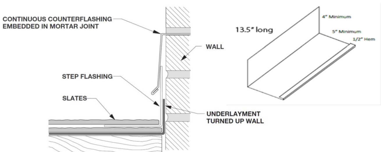
↑ Side Wall Step Flashing
