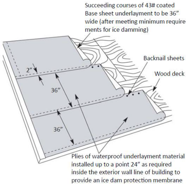
↑ Single Sheet Underlayment
