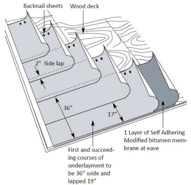
↑ Double Sheet Underlayment
